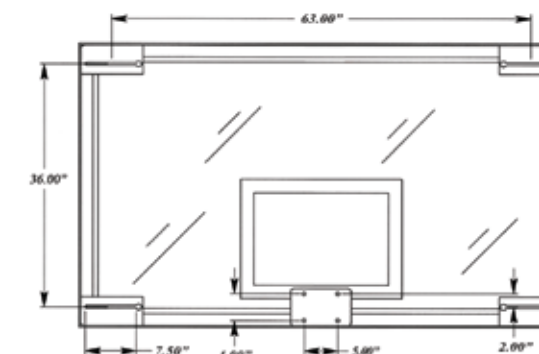
SuperGlass Collegiatesb Backboard 72" x 42"
